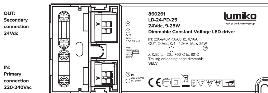
FIG. 1 CONNECTIONS
