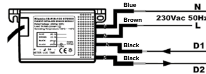
Fig. 3: Connection diagram
